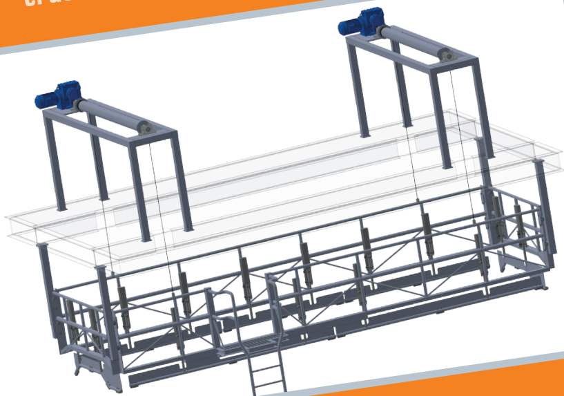
Mobile safety railing at the truck tanker filling points
